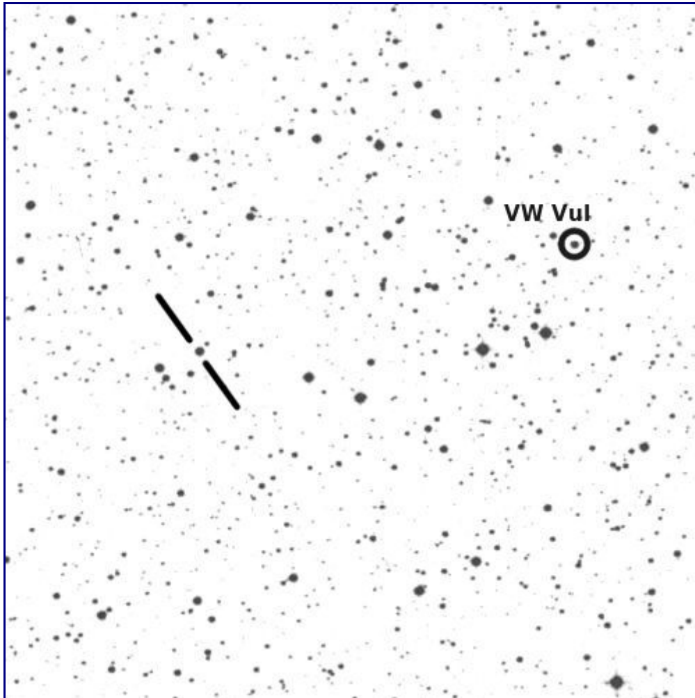
Finding chart of the new variable.
