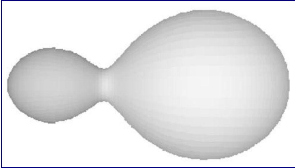
Geometrical representation of GSC2.3 N32O092280 during the maximum
