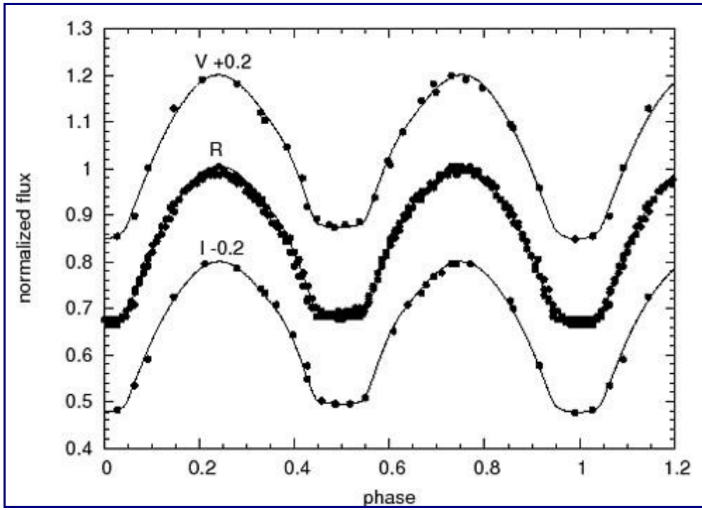
Comparison between theoretical (lines) and observed (circles) VR_C I_C phase diagrams of the new variable system in Vulpecula. The best fit is obtained with the Wilson-Devinney code for an A-type W UMa over-contact binary.
